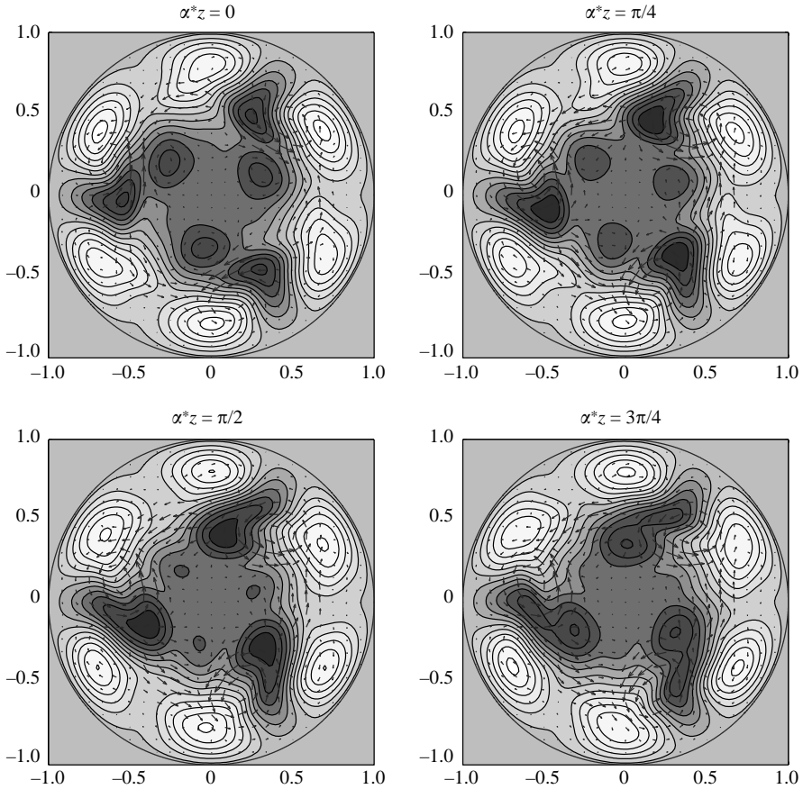
FIGURE 16. As figure 15 but for the \mathcal{R}_3 travelling wave solution at the saddle-node bifurcation \alpha^* = 2.44 and Re = 1250.9 . The 12 contour levels used range from -0.15 to 0.15 ). Notice that the slow interior streaks move around whereas the fast outer streaks are fairly stationary.
