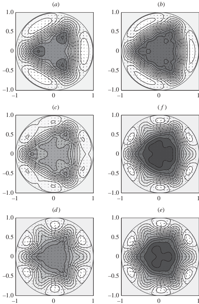
FIGURE 8. Streamwise-averaged plots of the various solutions labelled in figure 6 to show their different streak structure. The arrows indicate the streamwise-averaged cross-stream velocities \overline{v}_\perp^z (larger arrows corresponding to larger speeds) and the shading represents the streamwise-averaged axial velocity differential, \overline{w}^z (dark most negative and light most positive; the shading of the area exterior to the pipe represents zero). Solutions are arranged in branch pairings – a and b , c and f , and d and e – and so that the respective upper (lower) branch solution (referring to figure 7) is on the left (right). Since all solutions correspond to Re = 2200 the contour levels are kept constant across the figures (from -0.5 to 0.5 in steps of 0.031 ) to highlight their relative magnitude of \overline{w}^z . Quantitatively, (\min(\overline{w}^z), \max(\overline{w}^z), \max(|\overline{v}_\perp^z|)) = (-0.31, 0.057, 0.011) for a , (-0.33, 0.047, 0.018) for b , (-0.25, 0.037, 0.015) for c , (-0.28, 0.065, 0.013) for d , (-0.39, 0.068, 0.017) for e and (-0.40, 0.059, 0.020) for f (a speed of 1 corresponds to the centreline speed of the laminar solution at a Reynolds number of Re ).
